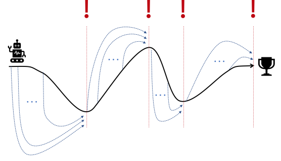
Figure 7.4: Keyframe selection and demo augmentation, where the black line represents a trajectory, '!' represents keyframes, and dashed blue lines represent the augmented transitions to the keyframes.
