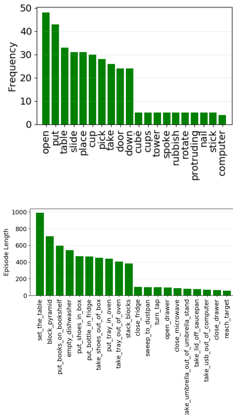
Figure 6.7: Top shows the 10 most and 10 least frequent words in the variation descriptions with function words removed, leaving only content words. Bottom shows the average length of 5 demonstrations from a sample of 20 tasks (taken from the first variation). The tasks lengths vary from 100 to 1000 timesteps. Longer tasks usually involve many composed sets of actions, for example, the ‘empty_dishwasher’ task involves opening the washer door, sliding out the tray, grasping a plate, and then lifting the plate out of the tray. These long-horizon tasks can facilitate interesting research in reinforcement learning in robotic tasks.
