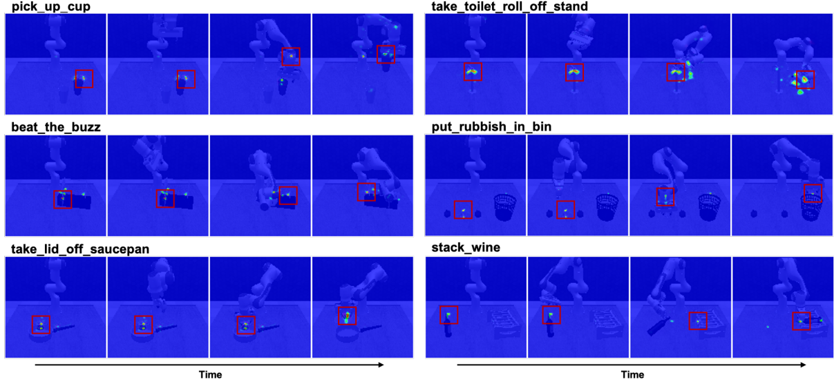
Figure 7.3: Visualising the Q values across 4 different points in time on 6 tasks. At each step, RGB and organised point cloud crops are made by extracting pixel locations that have the highest Q-value; crops are shown via the red squares. We can see that as time progresses, the attention strength shifts depending on progress in the task; e.g. ‘stack_wine’ starts with high attention on the bottle, but after grasping, attention shifts to the wine rack.
